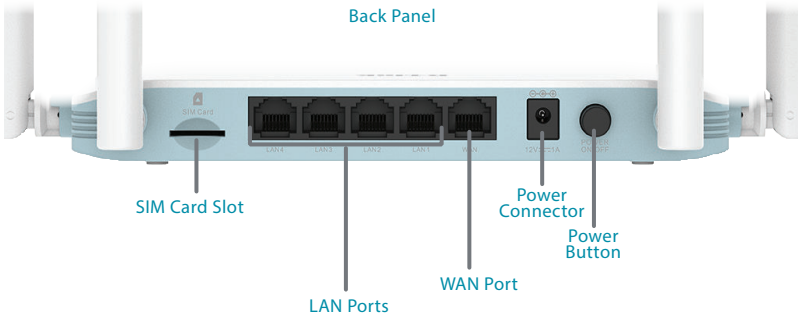
Back Panel
