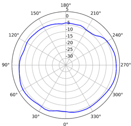
2.4GHz (Horizontal)
